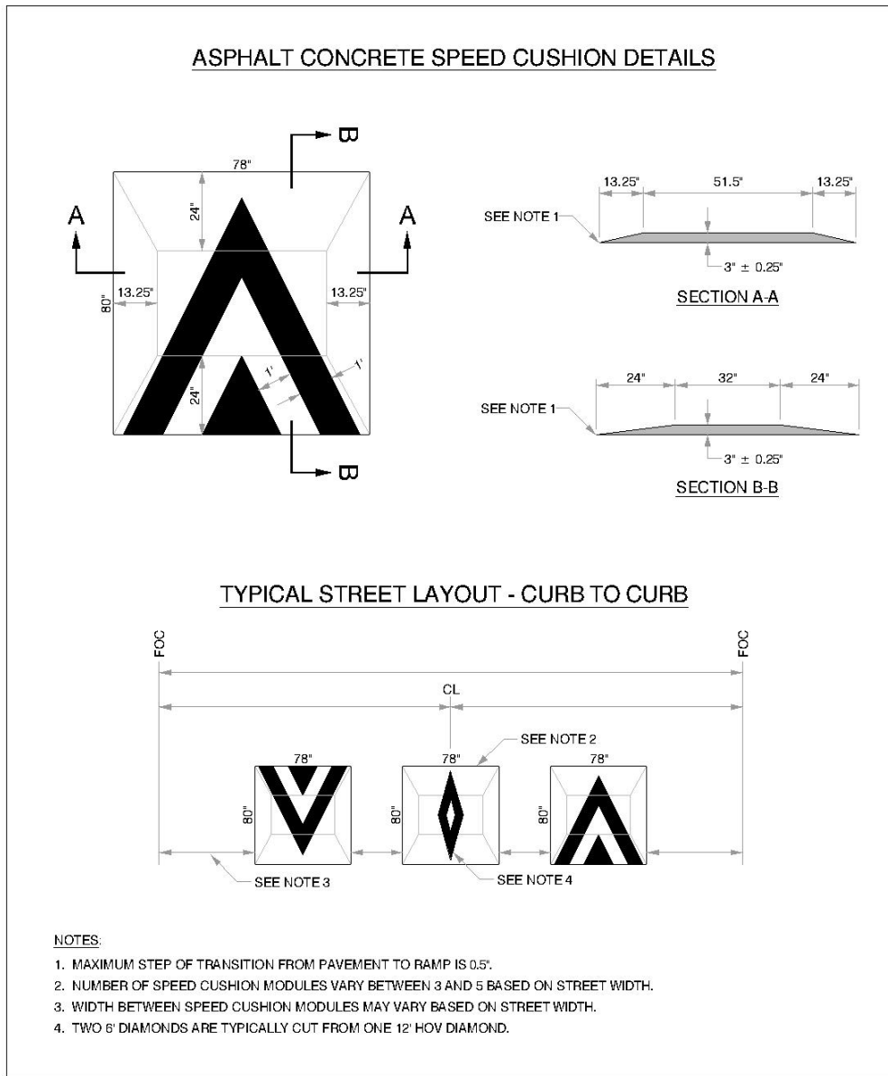
Figure A-10: Speed Cushion
